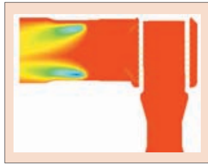
Figure 2: CFD Model of Steam Temperature Profile (left)
