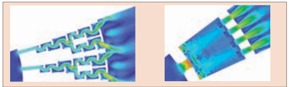
Figure 1: Velocity Profile of Tortuous Path Trim (Left) vs. WhisperFlo Trim (Right)
