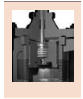
Figure 3: Example of Spring-type Pilot Balanced Valve Plug
