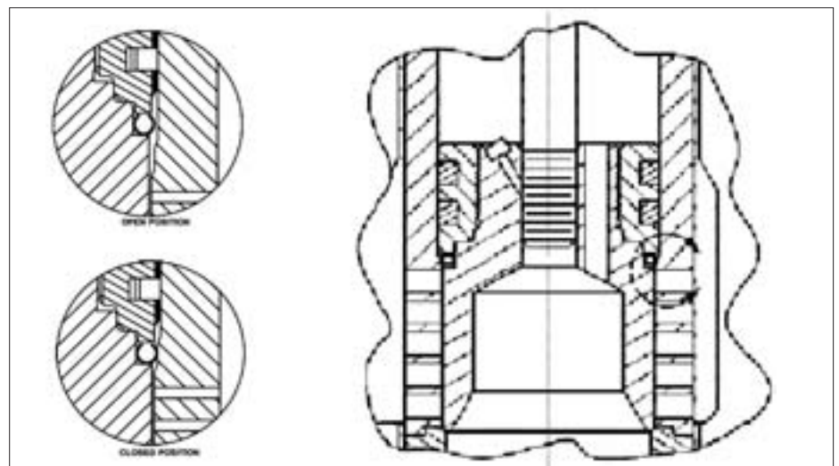
Figure 4: Cross Section of Balanced Trim with Tight Shutoff
