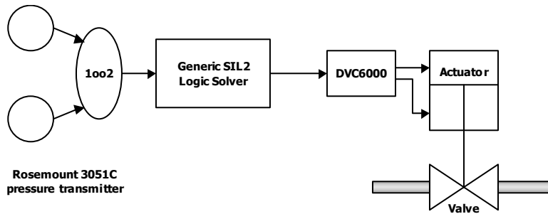
Figure 3 New conceptual design for SIF
