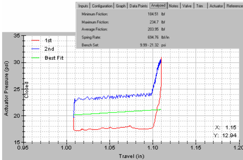
Figure 6 Valve signature used for diagnostics
