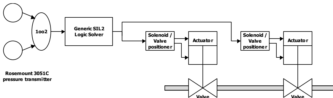
Figure 1 Conceptual design for SIL2 safety instrumented function
