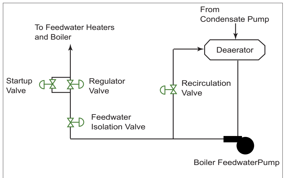
Figure 1. Schematic of a feedwater system
