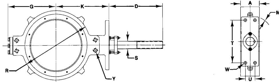
Figure 9. Dimensions and Weights, Wafer Style Valves, CL300 (also see table 5)
