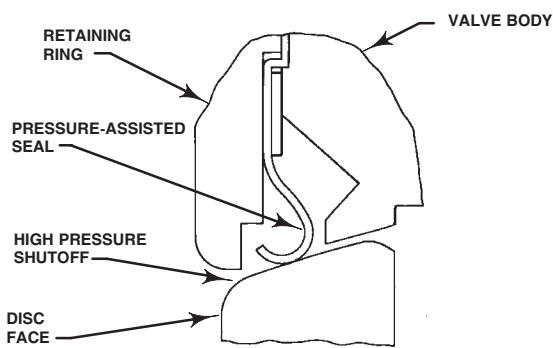
NPS 2 METAL SEAL
