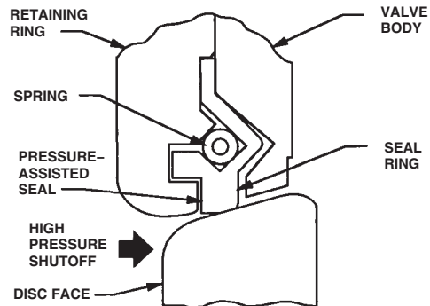
BIDIRECTIONAL SEAL PTFE, REINFORCED PTFE, AND UHMWPE SEALS
