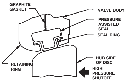
UNIDIRECTIONAL SEAL NOVEX METAL SEAL
