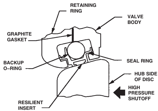
BIDIRECTIONAL SEAL PHOENIX III METAL SEAL
