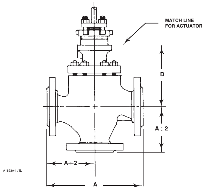
Figure 8. Fisher YD and YS Dimensions (also see table 9)
