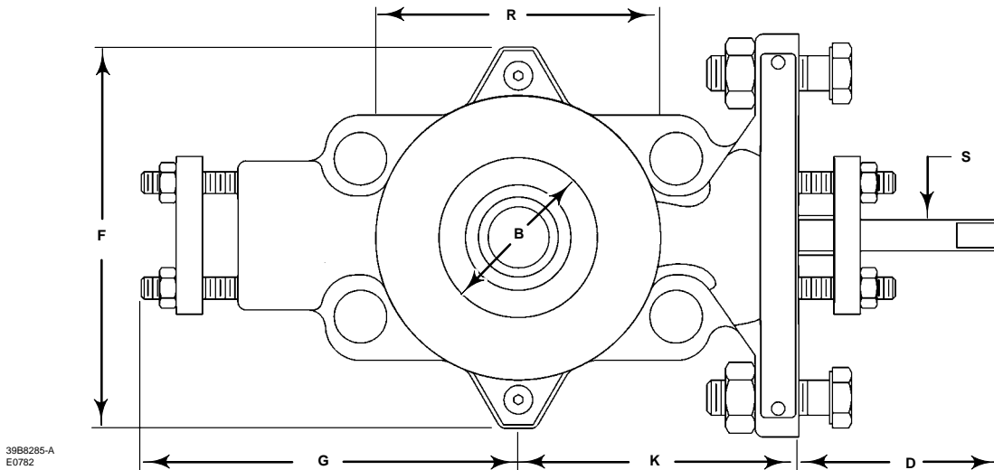
Figure 10. Dimensions for Type 8510B with Alternate Double D Shaft (also see table 14)
