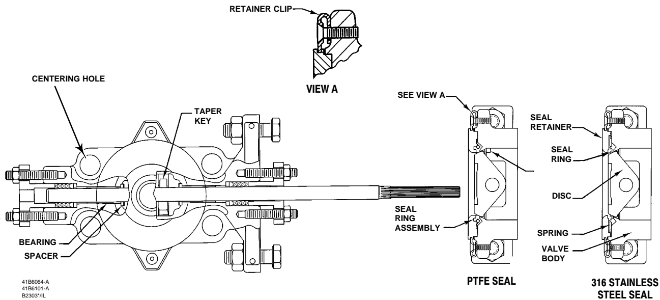
Figure 3. Typical Type 8510B Construction Detail
