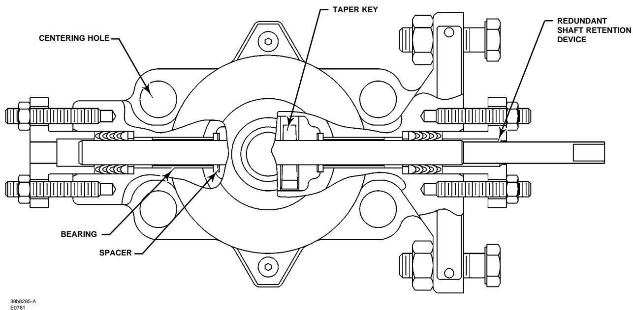
Figure 4. Typical Type 8510B Construction Detail with Double D Shaft
