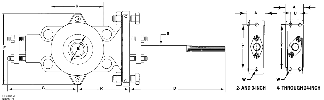
Figure 9. Dimensions for Type 8510 and 8510B (also see tables 12 and 13)
