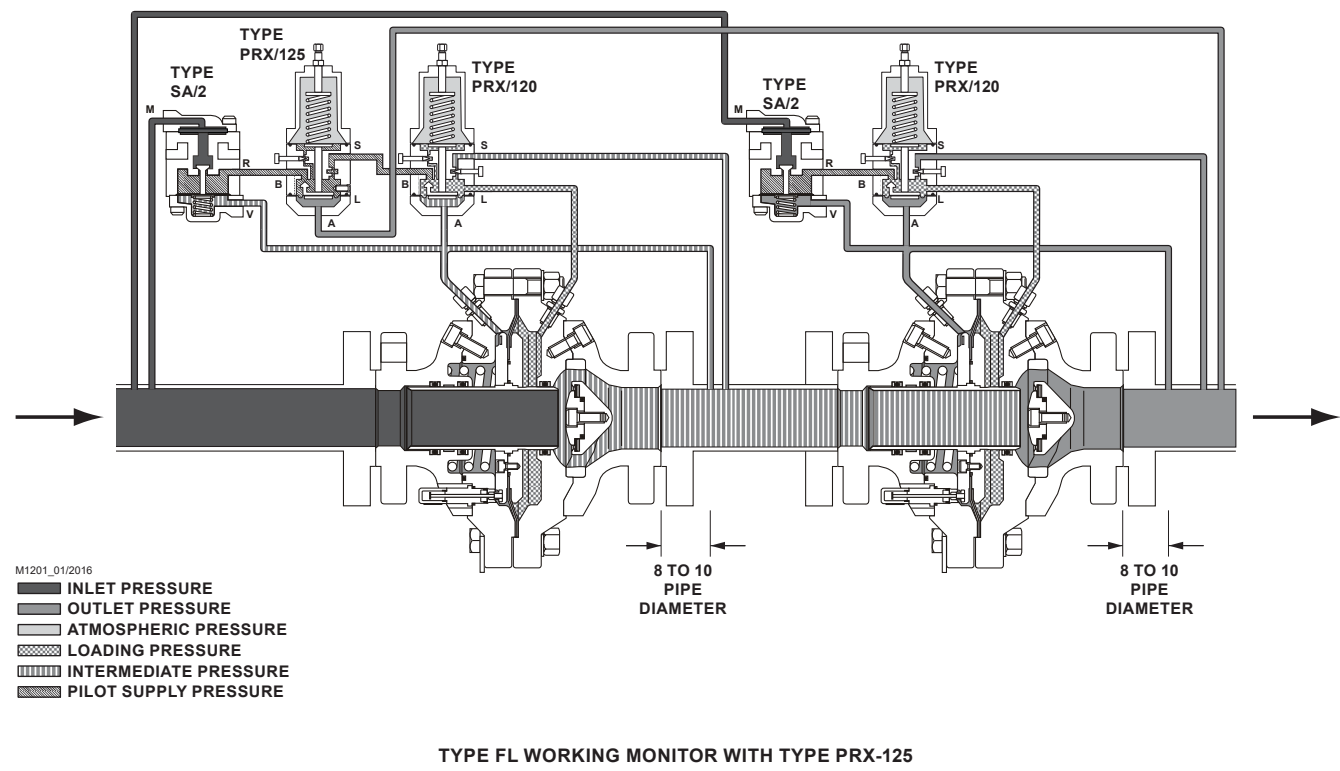
Figure 5. Typical FL Installation Schematics
