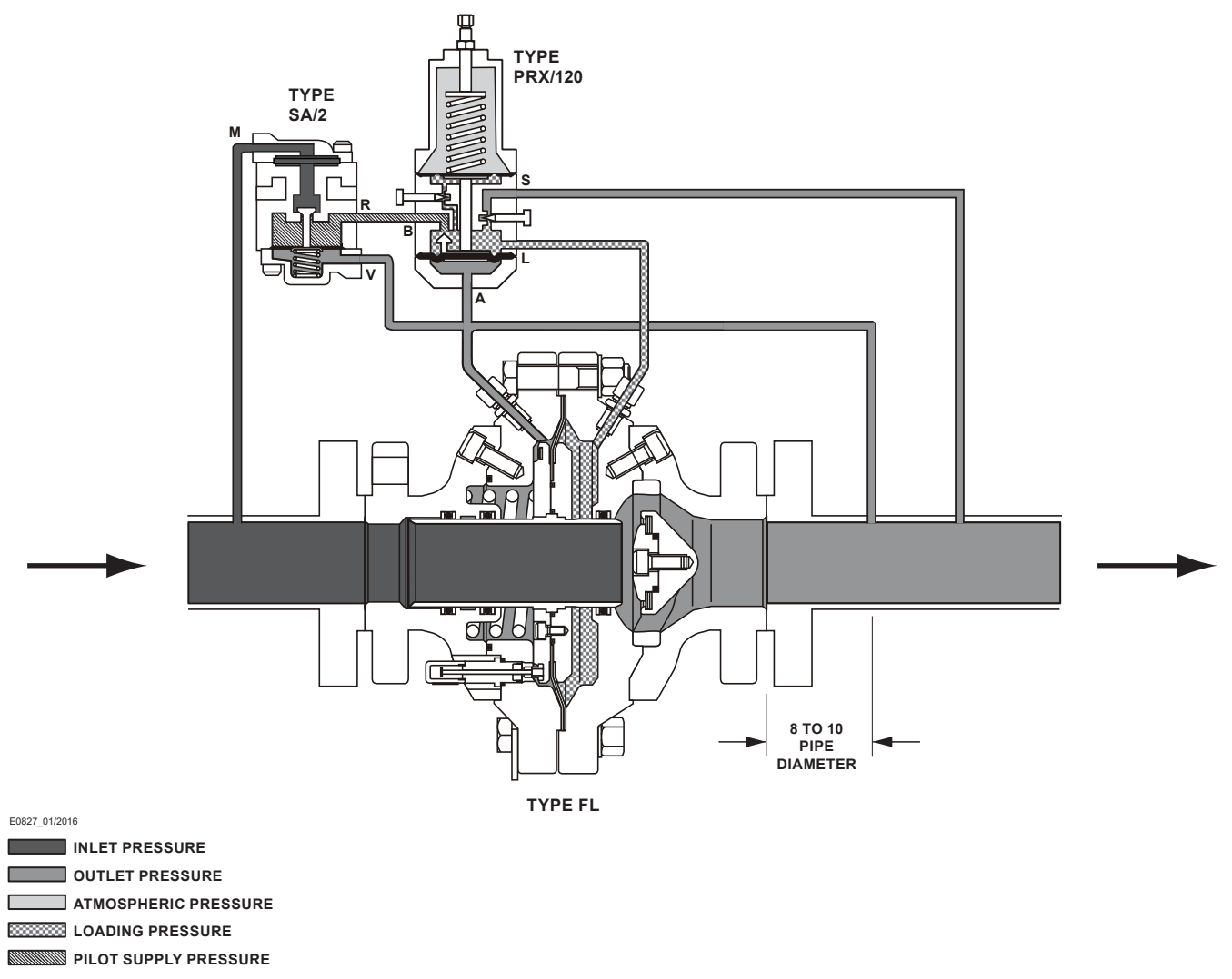
Figure 4. Type FL Operational Schematic
