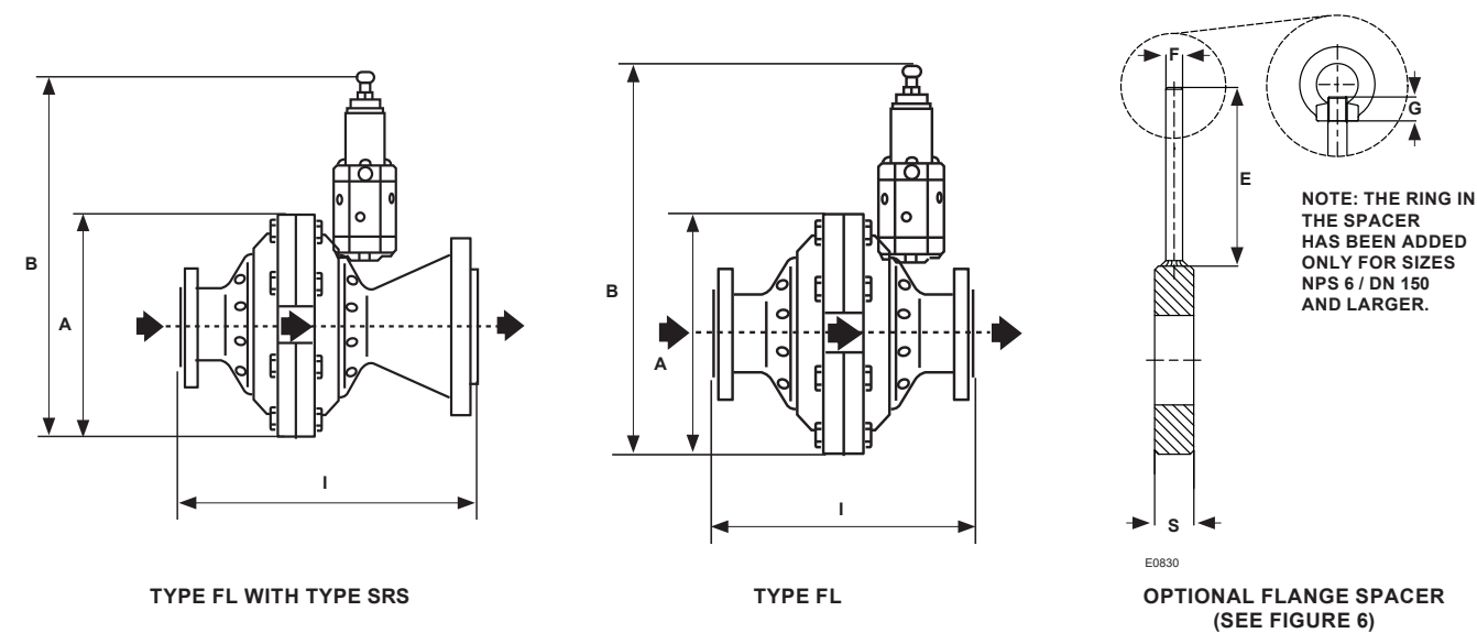
Figure 7. Dimensions
