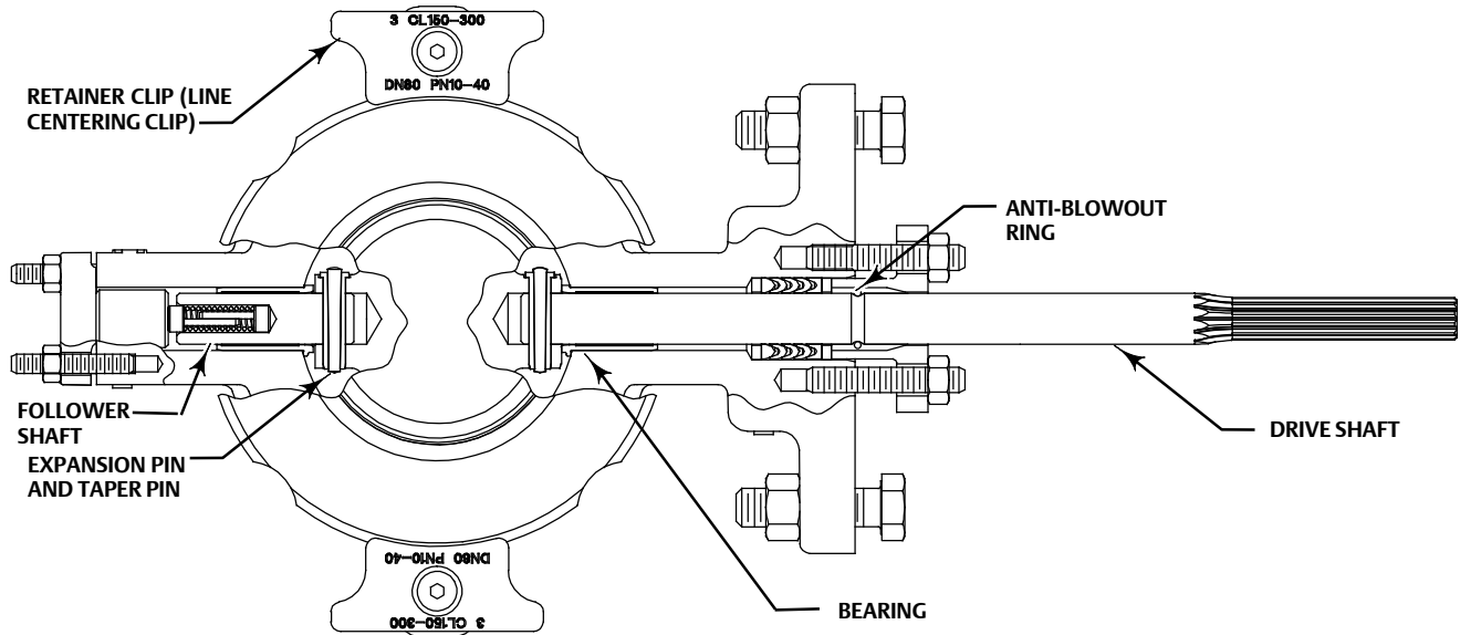
Figure 1. Typical Fisher 8580 Valve Construction Detail
