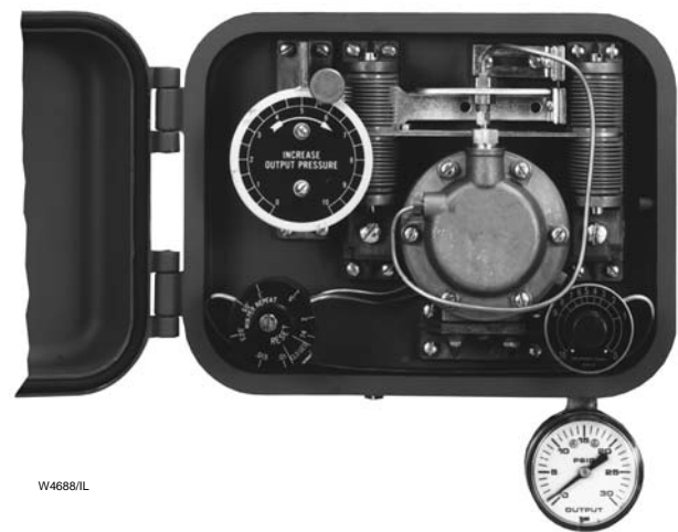
Figure 2. 2516 Receiver-Controller
