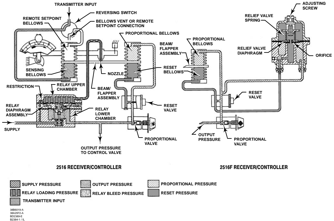
Figure 5. 2516 Receiver-Controller Schematic
