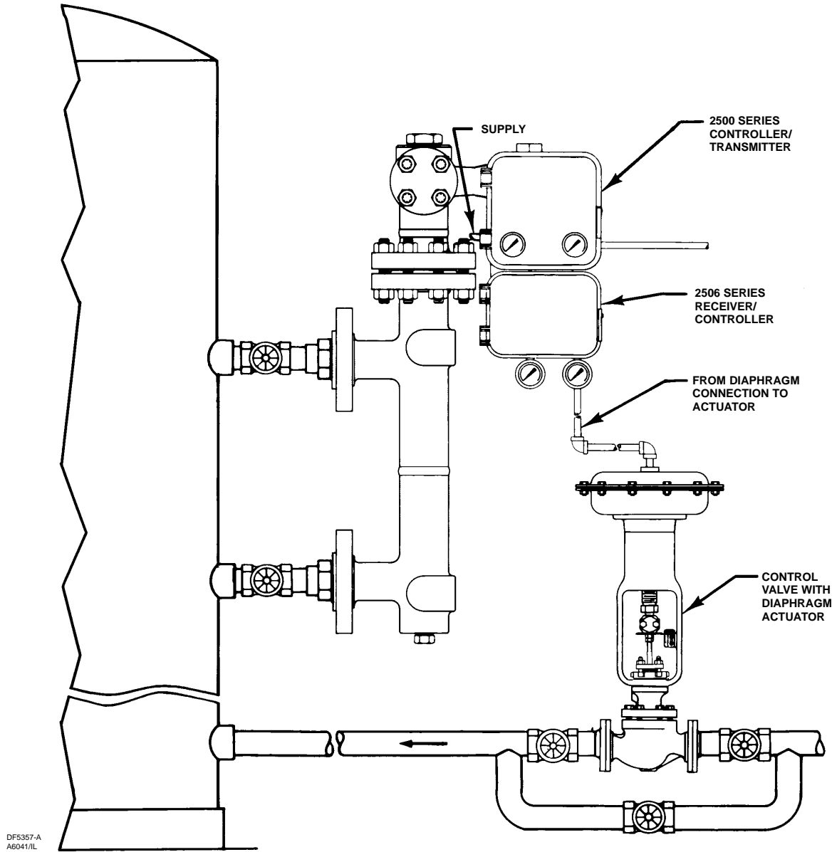
Figure 6. Receiver-Controller Mounted on a 2500 Series Controller/Transmitter
