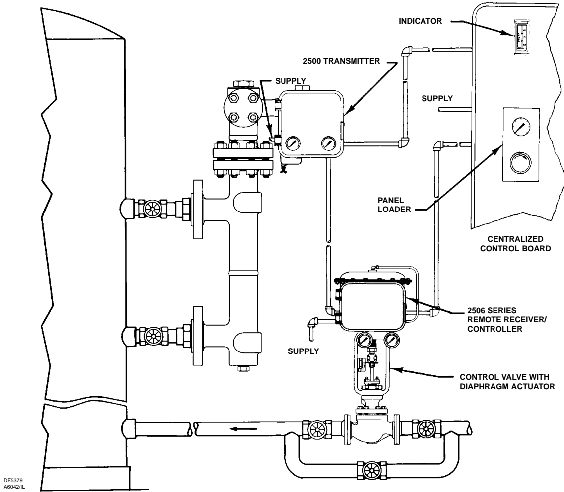
Figure 8. Receiver-Controller Mounted on the Actuator Yoke
