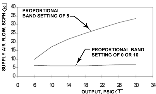
0.4 TO 2.0 BAR (6 TO 30 PSIG) OUTPUT SIGNAL RANGE
