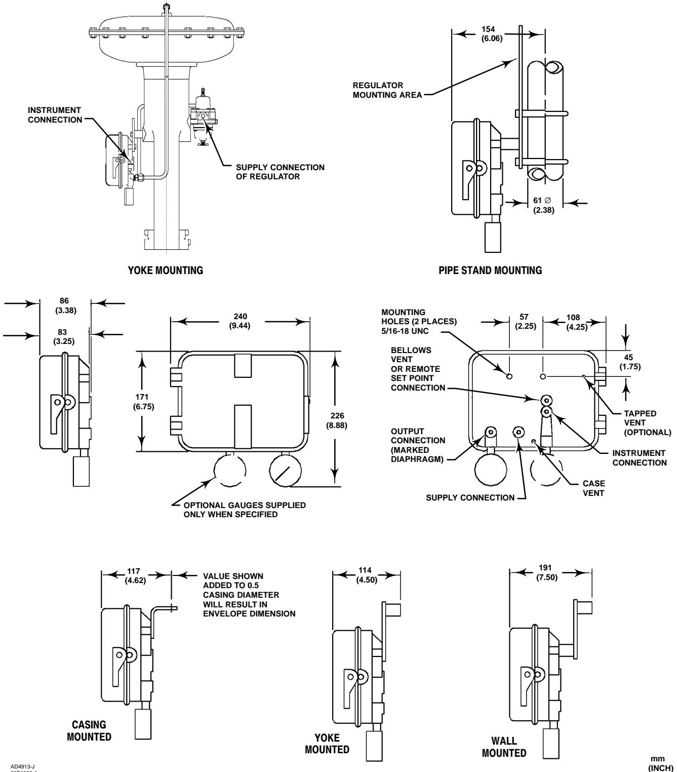
Figure 7. Dimensions
