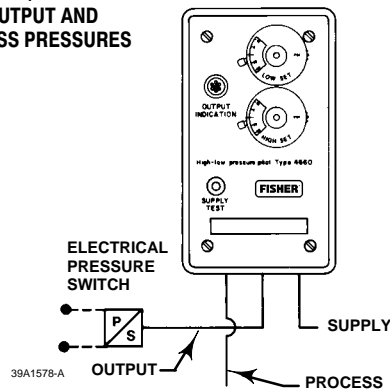
Figure 4. Typical Connection Schematics
