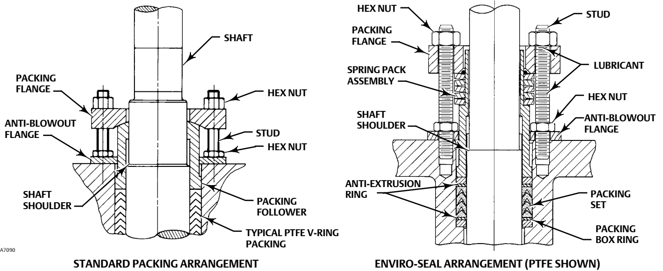
Figure 3. Blowout Protection
