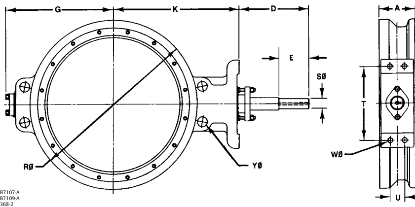
Figure 5. Dimensions and Weights, Wafer Style Valves, CL150 (also see table 2)
