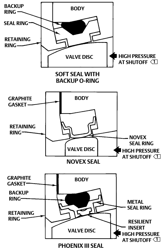
Figure 1. Available Seal Configurations
