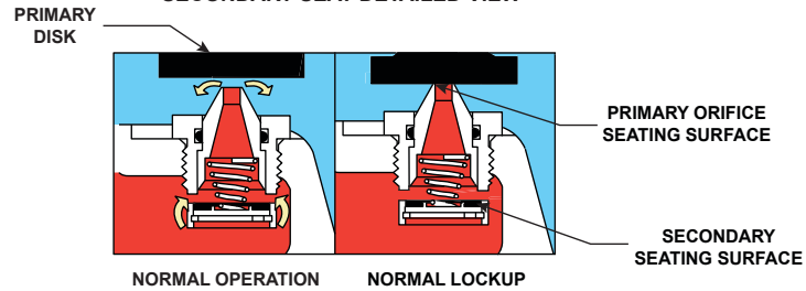
SECONDARY SEAT DETAILED VIEW
