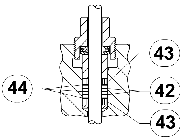
Figura 16. Gaxetas ULF Grafite ENVIRO-SEAL GX Fisher DN15 a DN100 (NPS 1/2 a 4)
