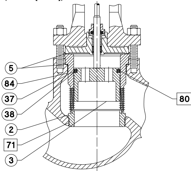
Figura 13. Internos Whisper Trim™ GX III Fisher (DN 150 [NPS 6])
