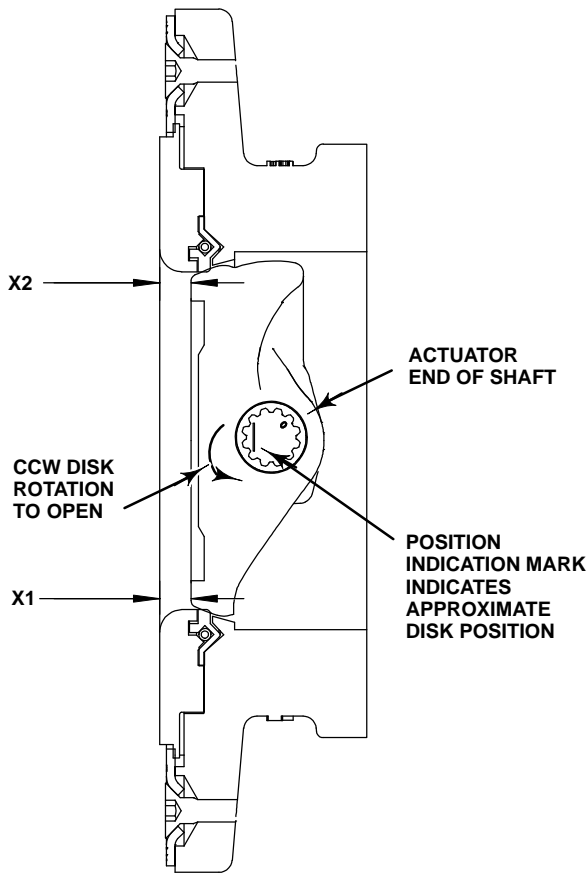
Figure 7. Sectional of Typical Valve Body
