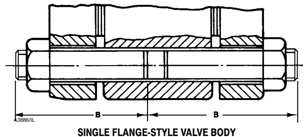
Figure 2. Stud Bolts for Installation (also see table 5)
