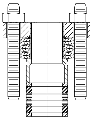
GRAPHITE PACKING ENVIRO-SEAL PACKING
