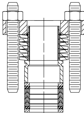
SINGLE PTFE PACKING
