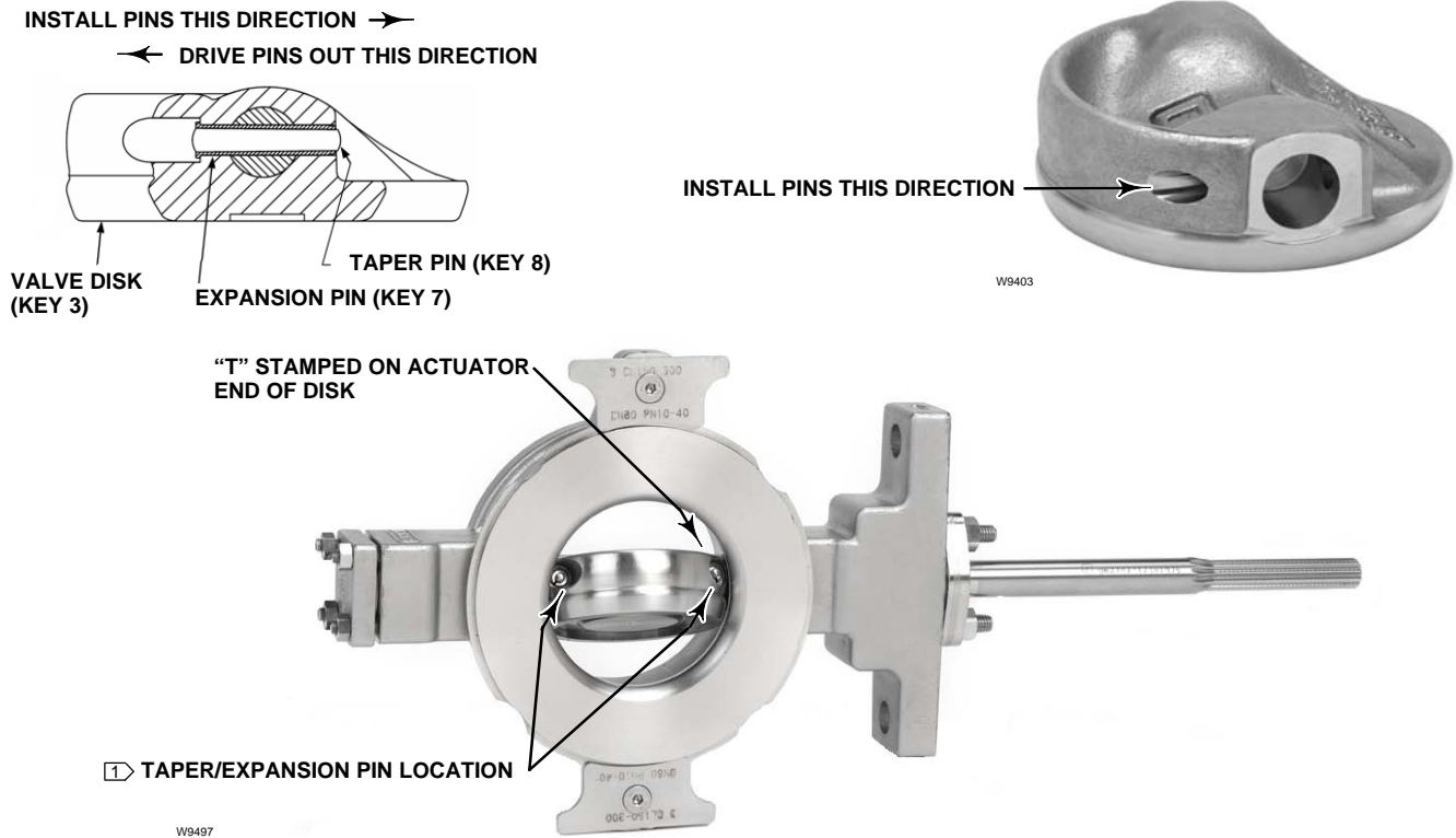
1. INSTALL THE PINS FROM THIS SIDE OF THE DISK.
