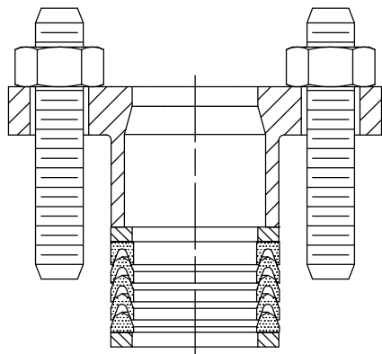
PTFE V-RING
