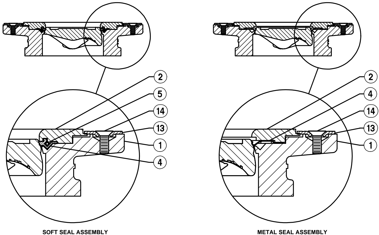
Figure 11. Fisher Control-Disk Seal Assembly Detail
