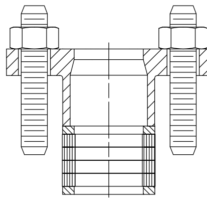
GRAPHITE RIBBON
