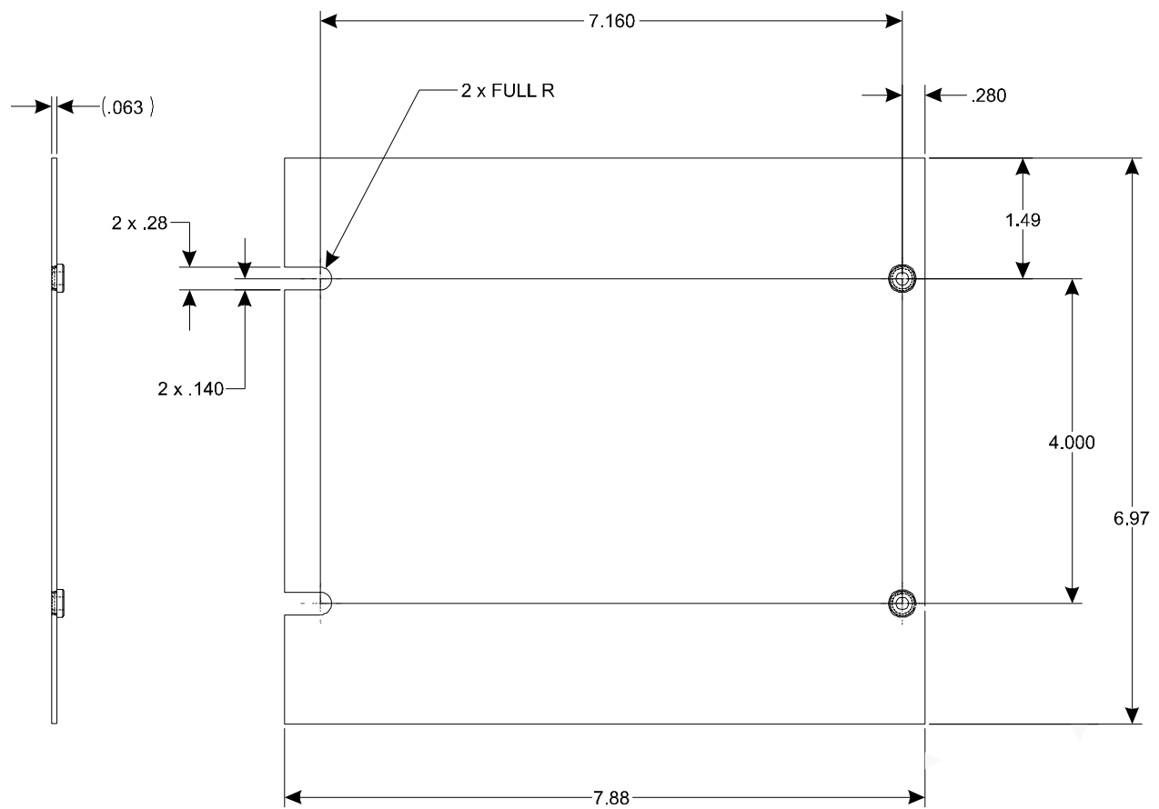
Figure 4-10 - ControlWaveRED Rack Mount Filler Panel Dimensions
