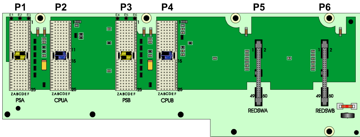
Figure 4-7 - Backplane PCB Connector Assignment
