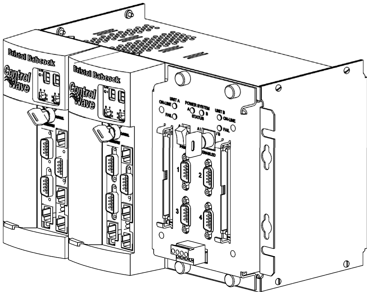
Figure 1-1 - ControlWaveRED Assembly
