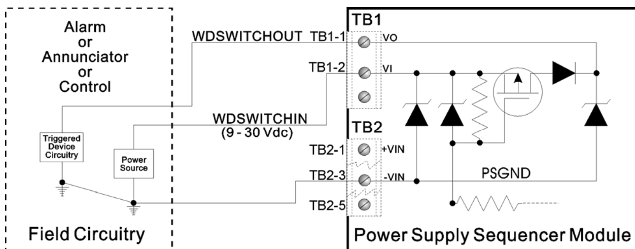
Figure 2-17 - Watchdog MOSFET Switch Field Wiring
