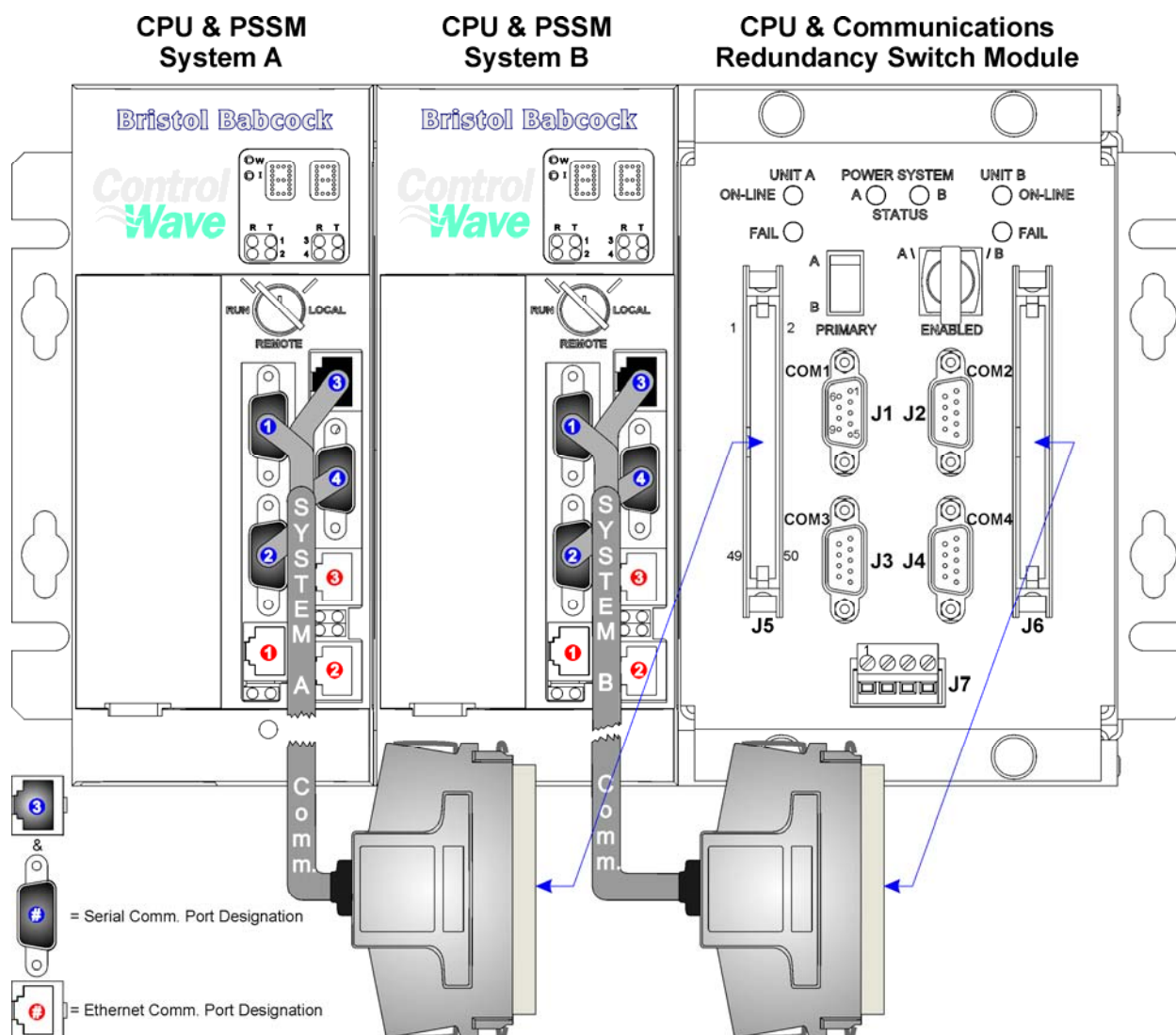
Figure 2-8 - Redundant Communication Cables Connection Diagram
