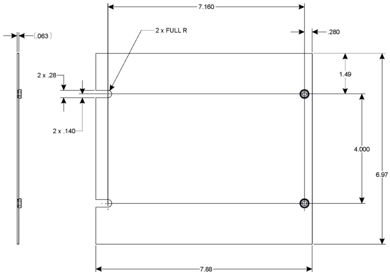
Figure 2-2 - ControlWaveRED Rack Mount Filler Panel Dimensions
