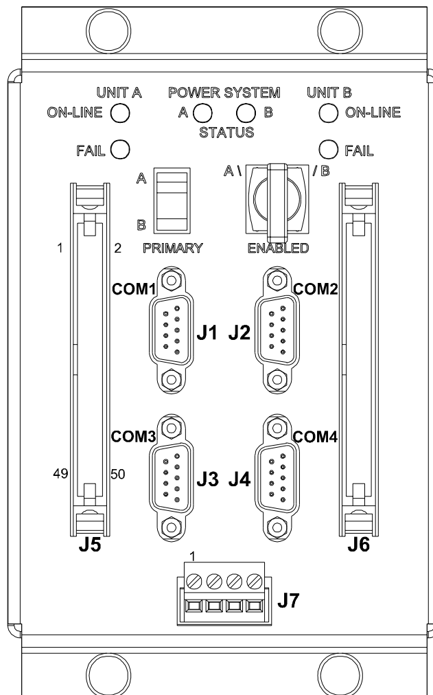
Figure 4-8 – CCRS Module Connector Assignment
