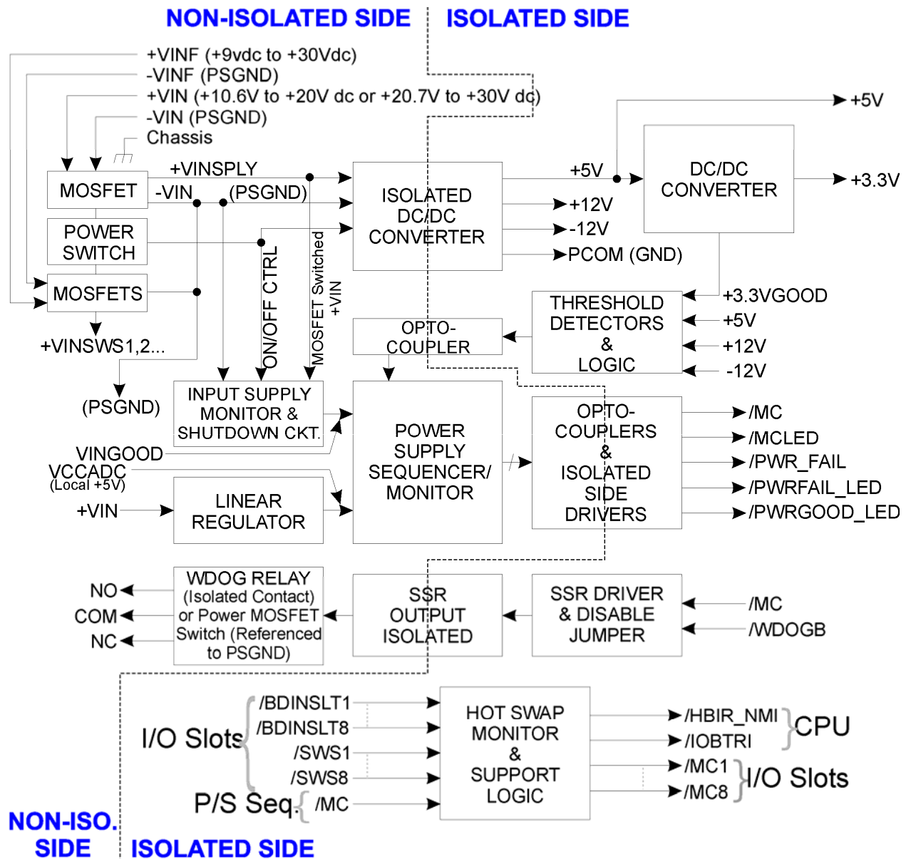
Figure 1-7 - Power Supply/Sequencer Module Block Diagram
