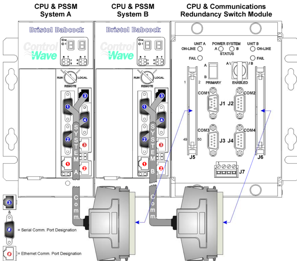
Figure 1-12 - ControlWaveRED Chassis and Comm. Cabling Diagram
