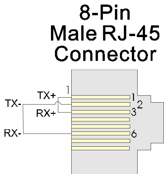
Figure 3-12 - RJ-45 Ethernet Loop-back Plug
