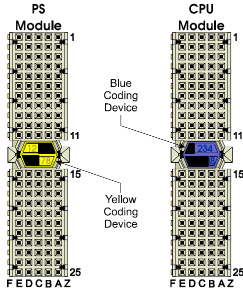
Figure 4-1 - Power Supply Bd. & CPU Bd. Backplane Connectors Looking into Board Connectors
