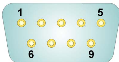
Figure 2-10 - Male DB9 9-Pin Connector (CPUM: COM1, COM2 & COM4) (CCRSM: COM1 - COM4)
