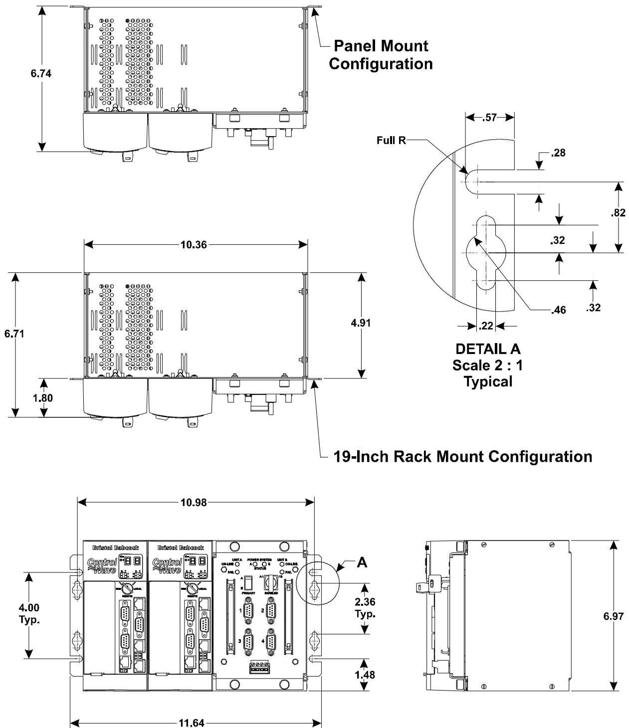
Figure 4-9 - ControlWaveRED Dimension & Installation Drawing
