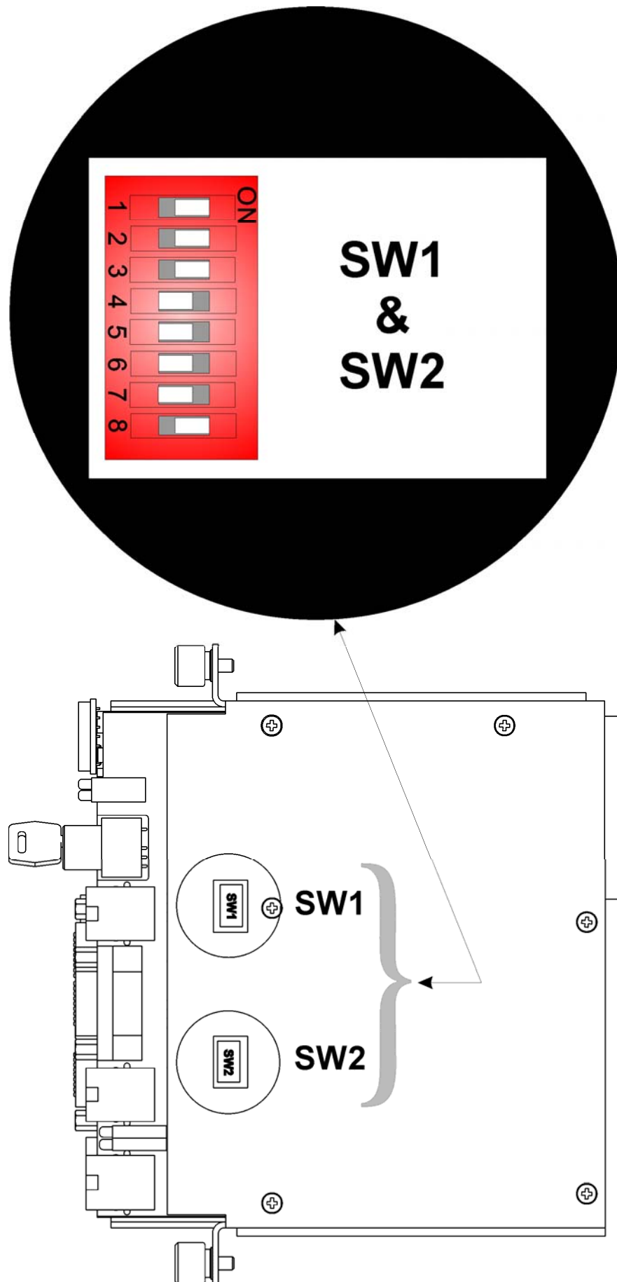
Figure 2-11 - Secondary Comm. Bd. Switches SW1 (COM3) & SW2 (COM4)
