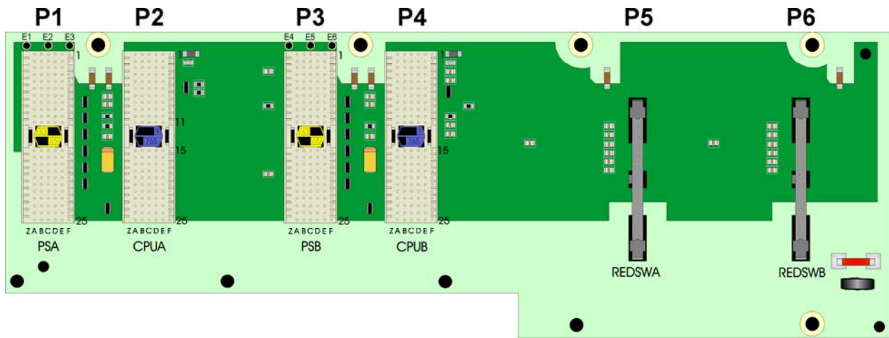
Figure 1-10 - ControlWaveRED Backplane Assembly
