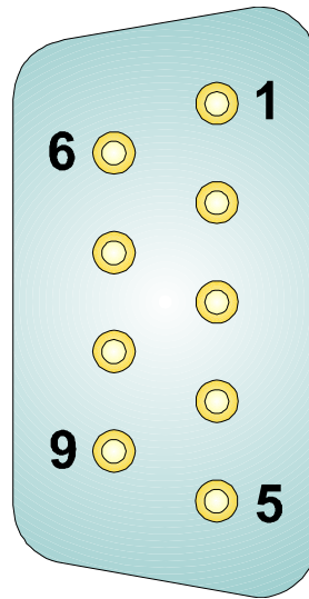
Figure 4-2 - DB9 9-Pin Connector Port Pin Assignments CPU Module Comm. Ports COM1, COM2 & COM4 CCRS Module Comm. Ports COM1, COM2, COM3 & COM4
