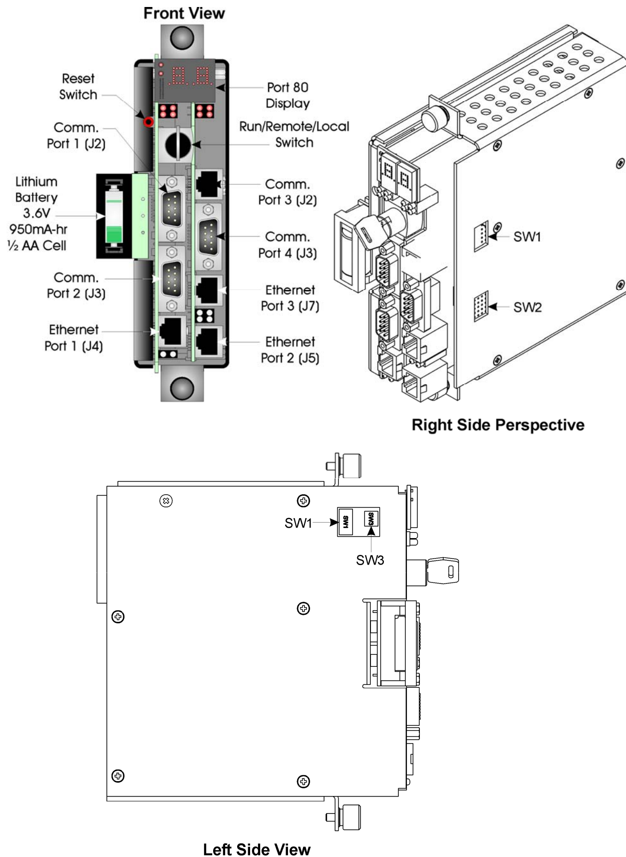
Figure 1-4 - ControlWaveRED CPU Module
