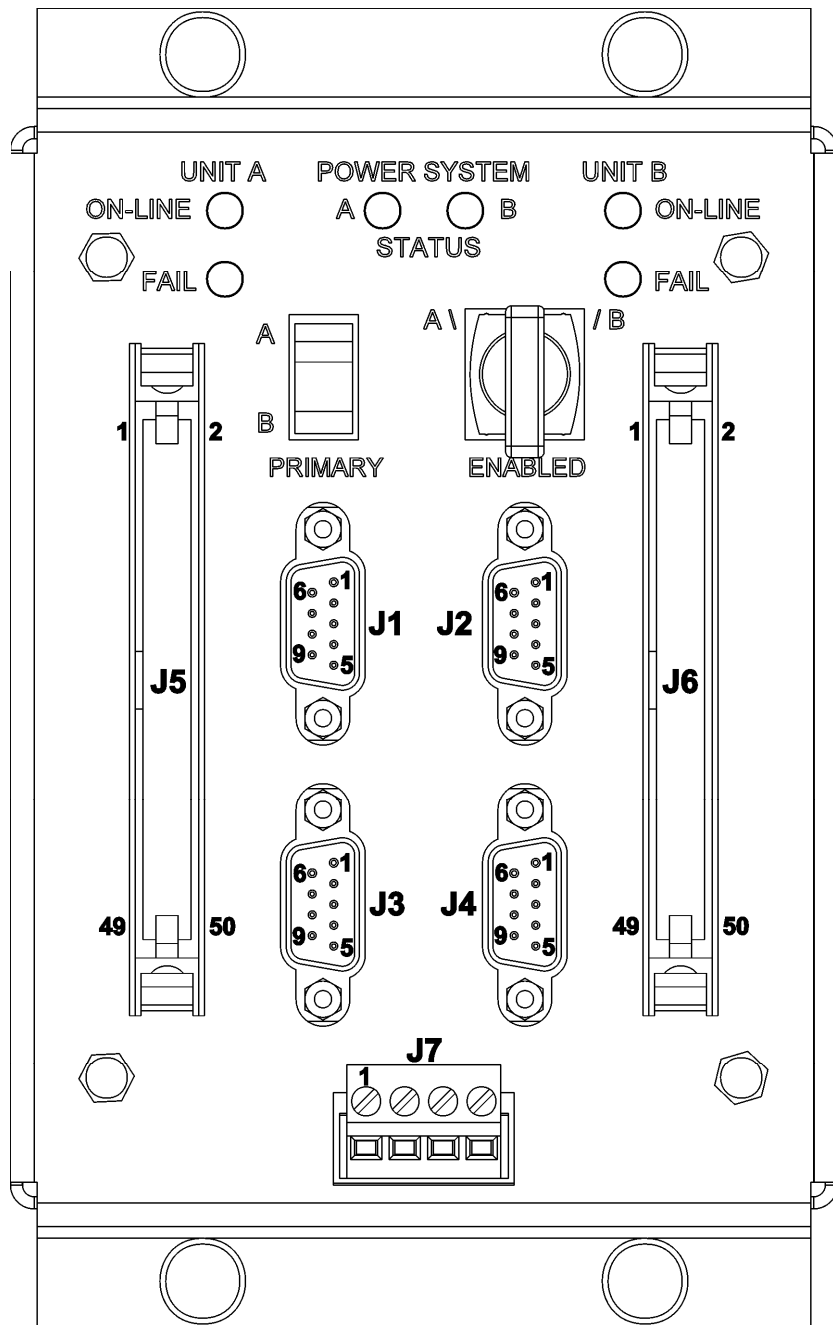
Figure 1-9 - Front View of CPU & Comm. Redundancy Switch Module
