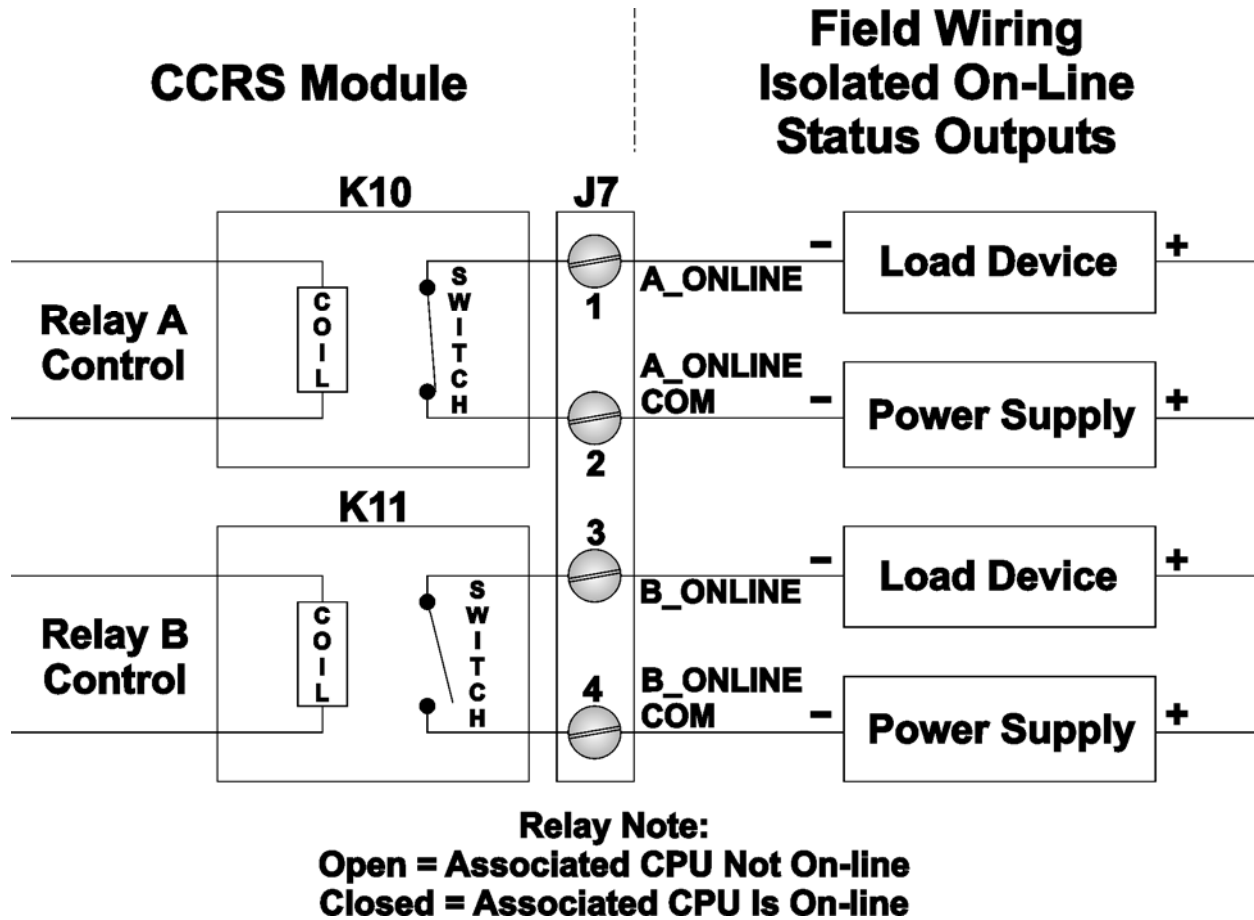
Figure 2-18 - CCRS Module - Isolated On-Line Status Outputs - Field Wiring
