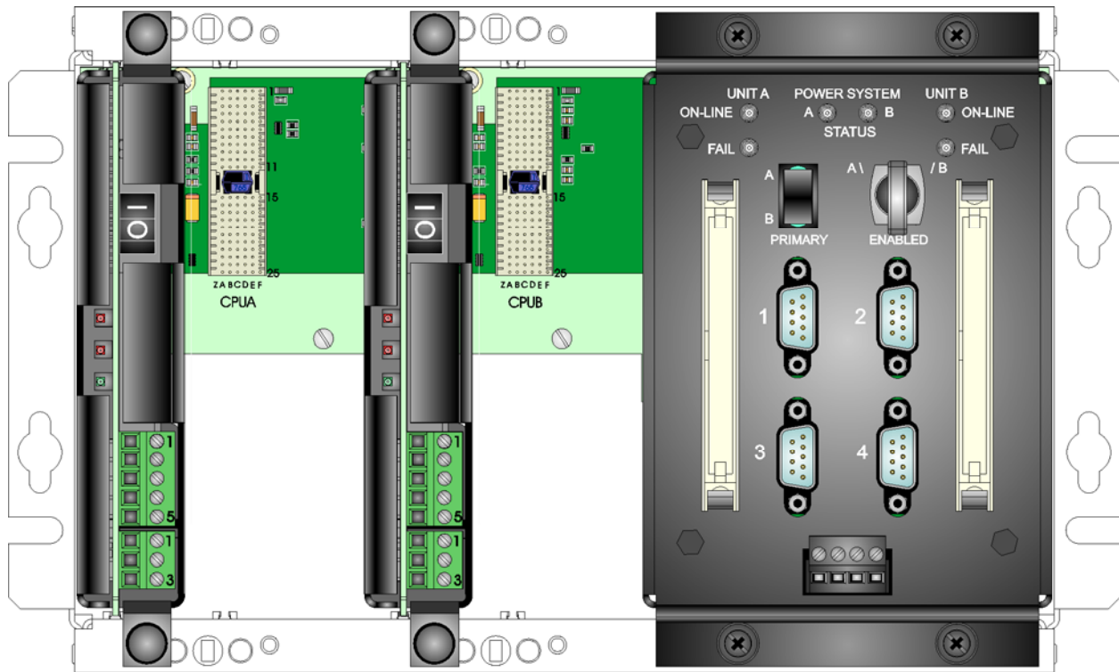
Figure 2-4 - PSSMs Installed in ControlWaveRED Slots #1 and #3
