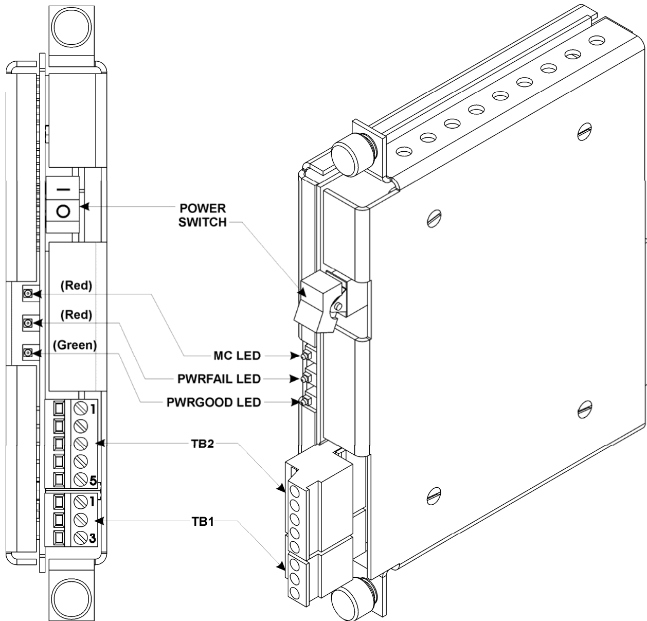
Figure 1-6 - Power Supply/Sequencer Module
