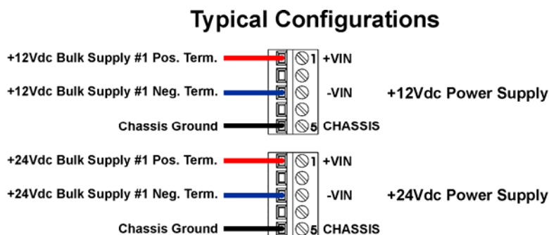
Figure 2-16 - PSSM TB2 Typical Wiring Schemes
