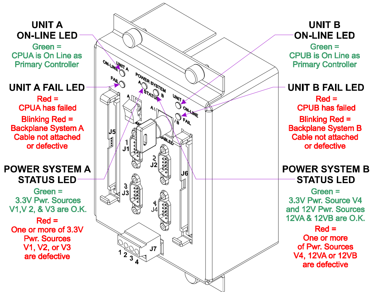
Figure 3-6 - CCRS Module LED Designations
