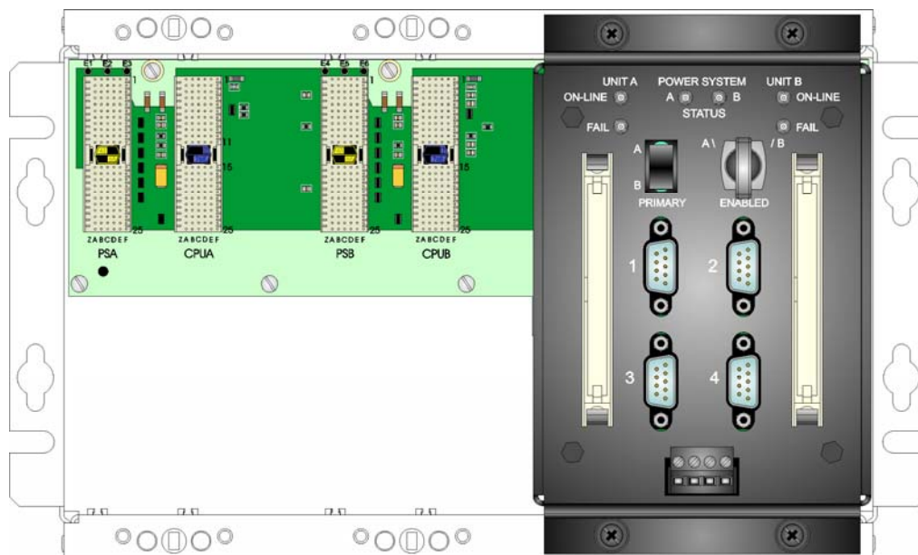
Figure 2-3 - ControlWaveRED Prior to Installation of PSSMs
