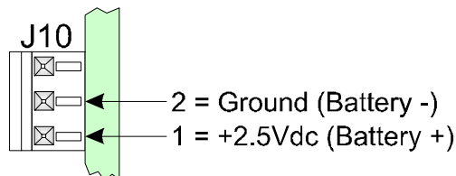
Figure 4-5 - Connector J10 - CPU Battery Header
