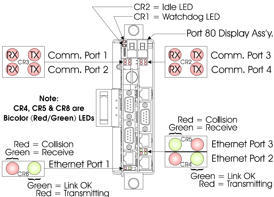
Figure 3-5 - CPU Module Port & LED Designations
