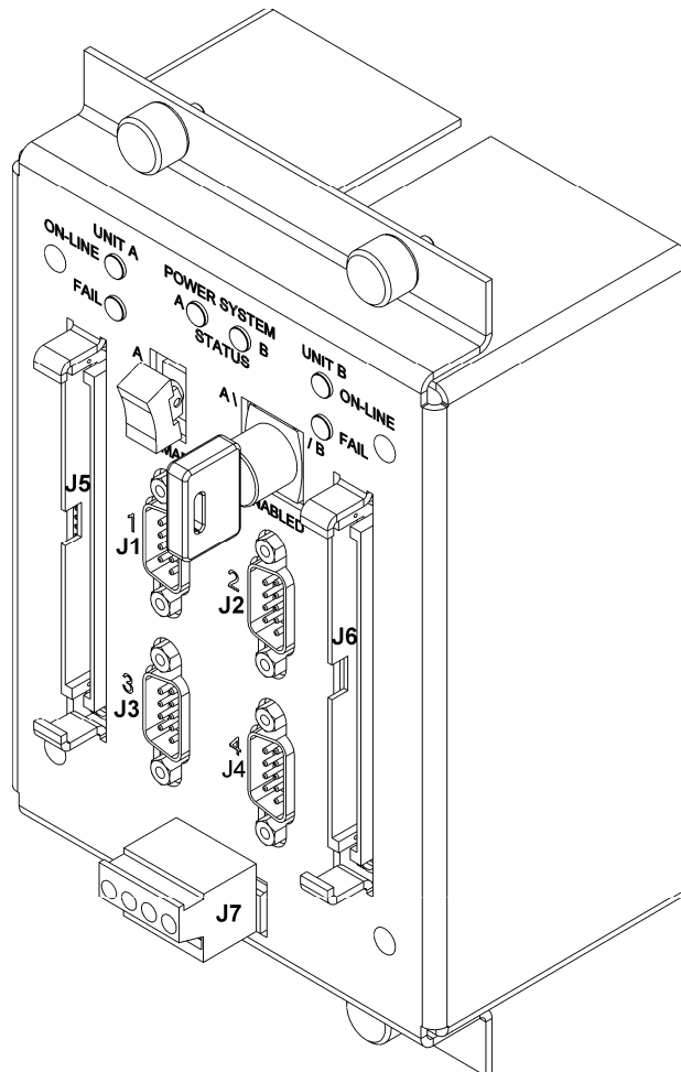
Figure 1-8 - Perspective View of CPU & Comm. Redundancy Switch Module
