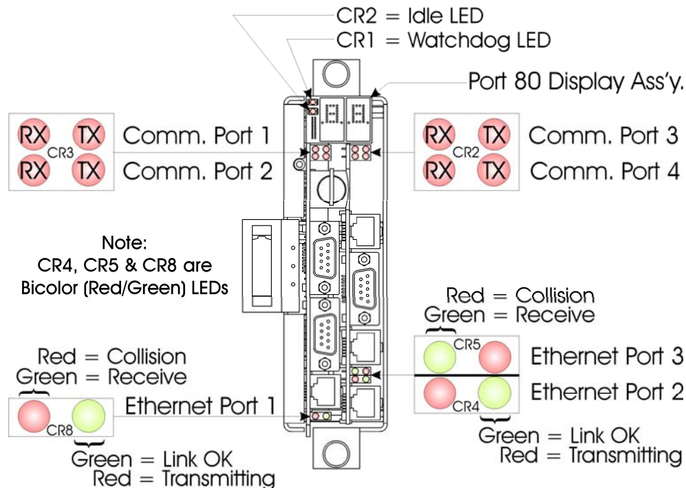
Figure 1-5 - CPU Module LEDs
