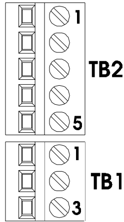
Figure 4-6 - Power Supply/Sequencer Module Connectors TB1 & TB2
