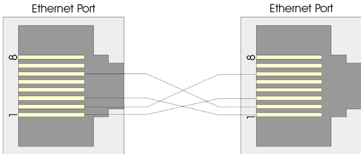
Figure 2-13 - Point-to-Point 10/100Base-T Ethernet Cable
