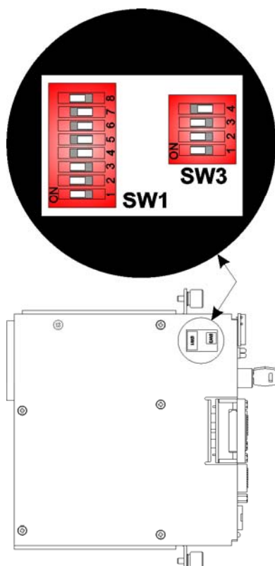
Figure 2-6 - CPU Module Switches SW1 & SW3
