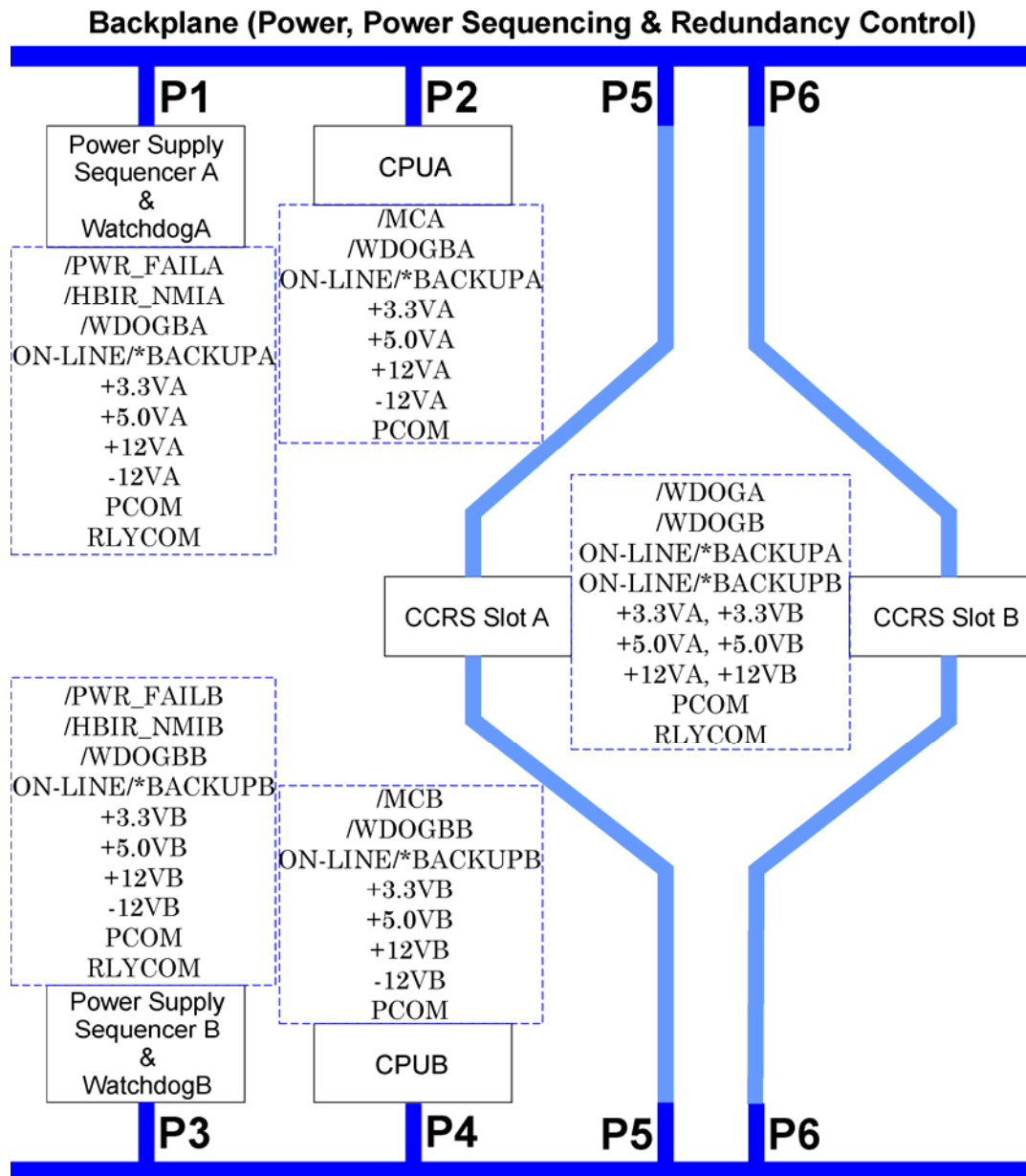
Figure 1-11 - Backplane PCB Block Diagram
