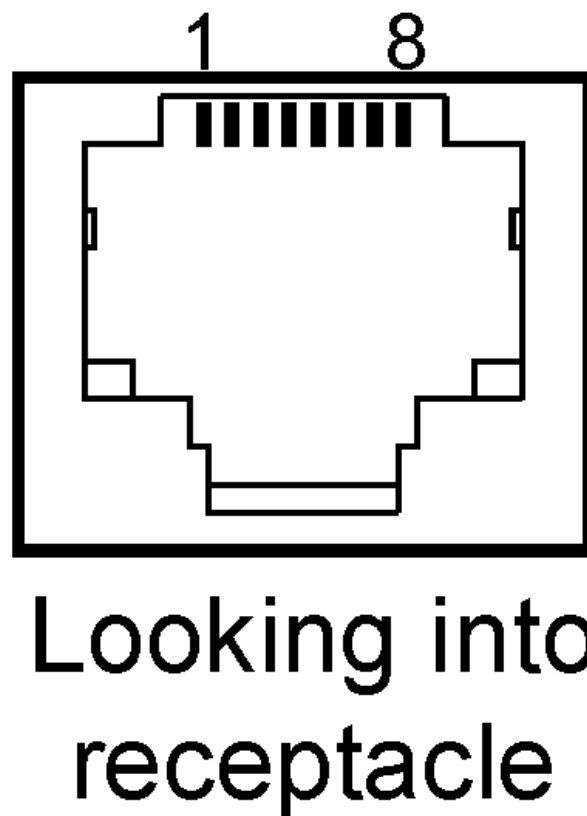
Figure 2-12 - RJ-45 Connector (Ethernet Ports) J2 (CPU), J5 & J7 (SCB)
