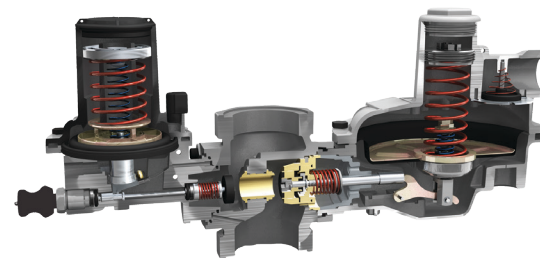
Typical CSB404 Regulator with Slam-shut Internal View
