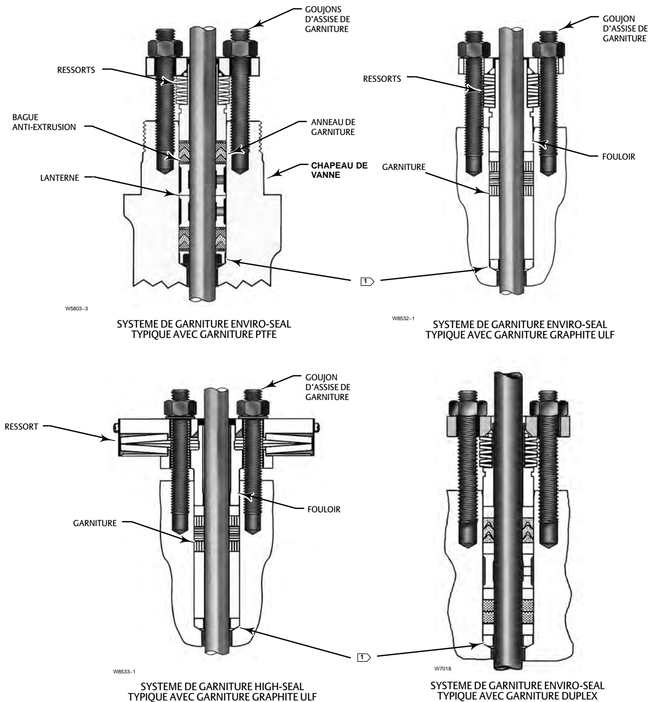
Figure 4. Systèmes de garnitures ENVIRO-SEAL et HIGH-SEAL
