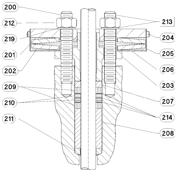
Figura 4. Baderna live-loaded
