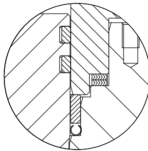
VISTA A TENUTA BORE SEAL, FLUSSO IN ALTO
