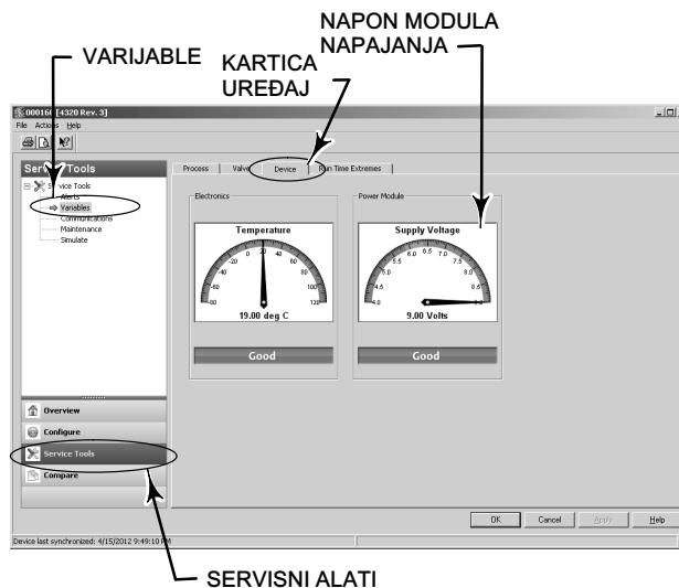
Slika 27. Status napajanja u programima AMS Wireless Configurator i AMS Device Manager
