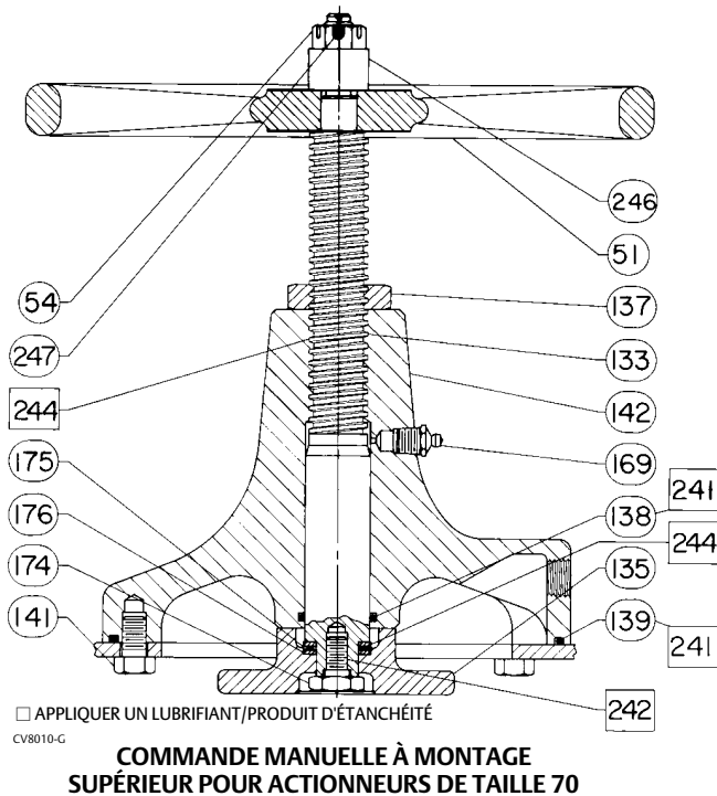
Figure 9. Commandes manuelles
