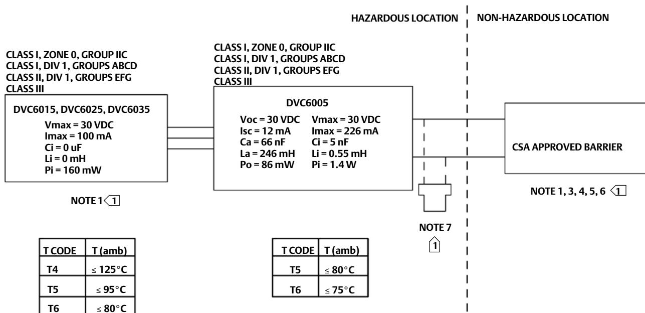
Figure 1. CSA Loop Schematics FIELDVUE DVC6005 HW1 and DVC6015, DVC6025, DVC6035
