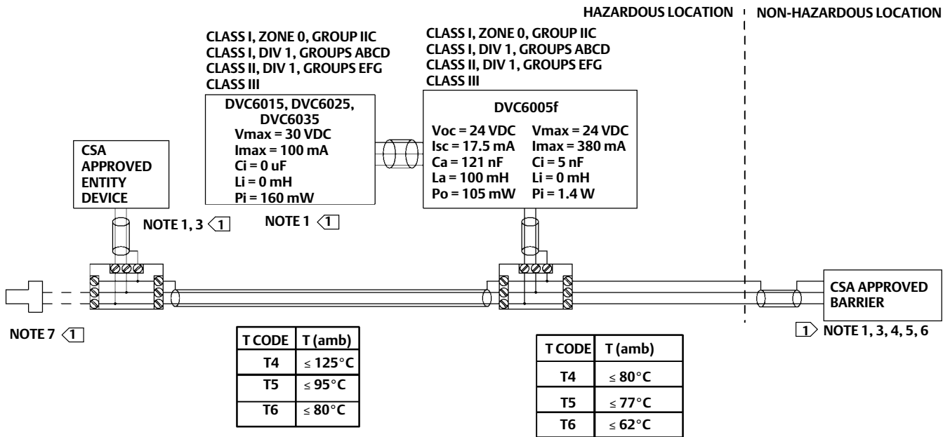
Figure 3. CSA Loop Schematics FIELDVUE DVC6005f and DVC6015, DVC6025, DVC6035
