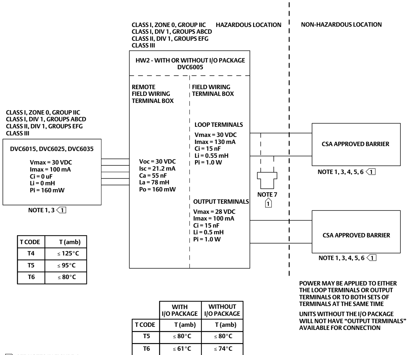
Figure 2. CSA Loop Schematics FIELDVUE DVC6005 HW2 and DVC6015, DVC6025, DVC6035
