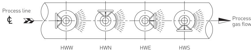
HANDWHEEL POSITIONS
