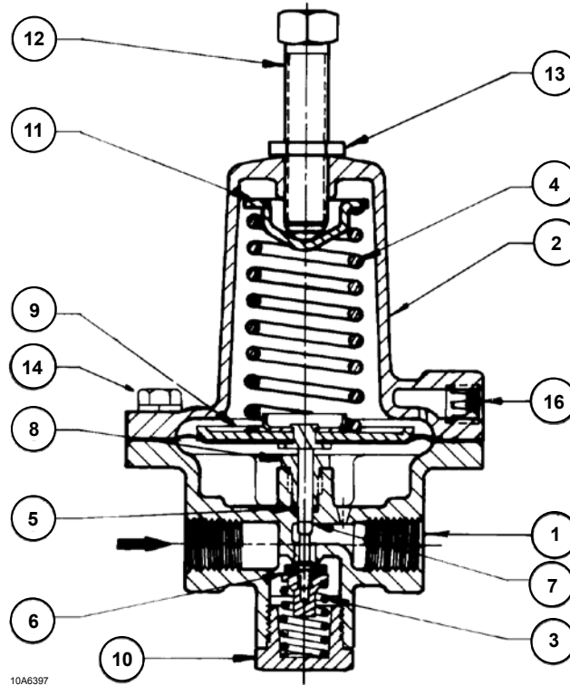
Figure 1. Type 64 LP-Gas Regulator Assembly
