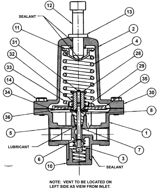
Figure 2. Type 64SR LP-Gas Regulator Assembly
